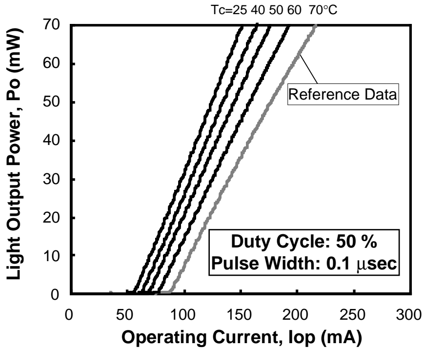
Light Output Power vs. Current (Pulse)
