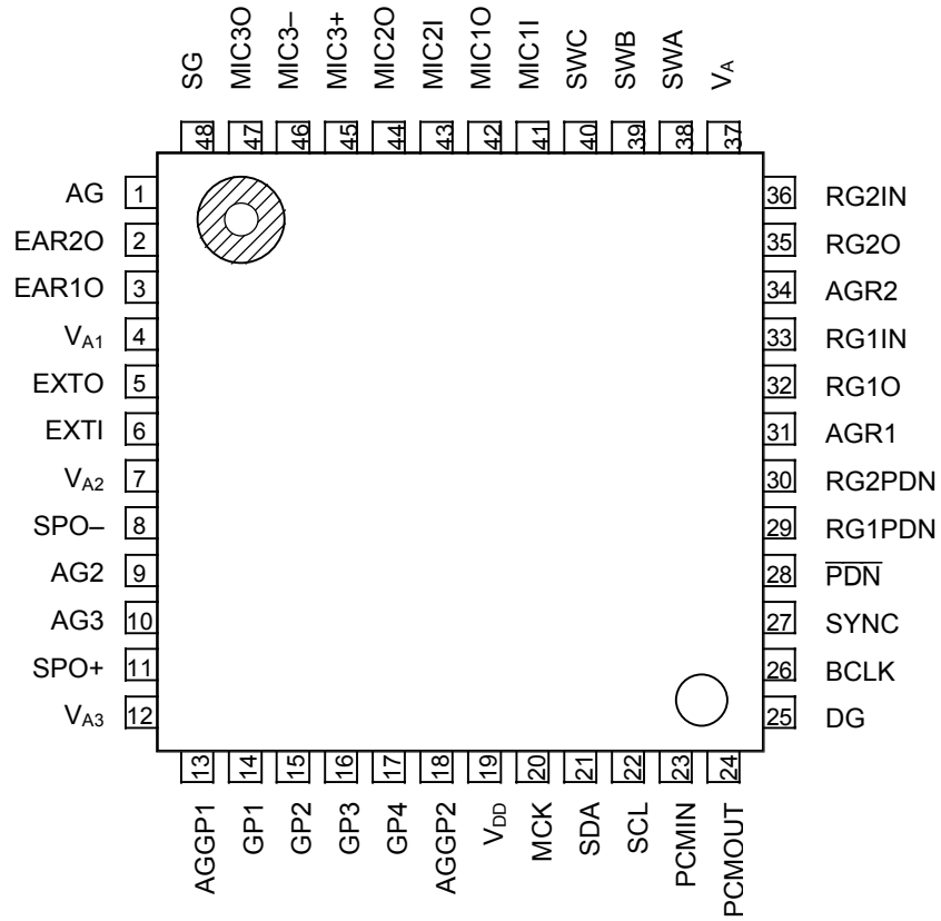
48-Pin Plastic TQFP
