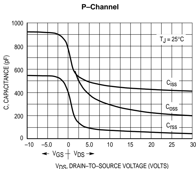
Figure 7. Capacitance Variation
