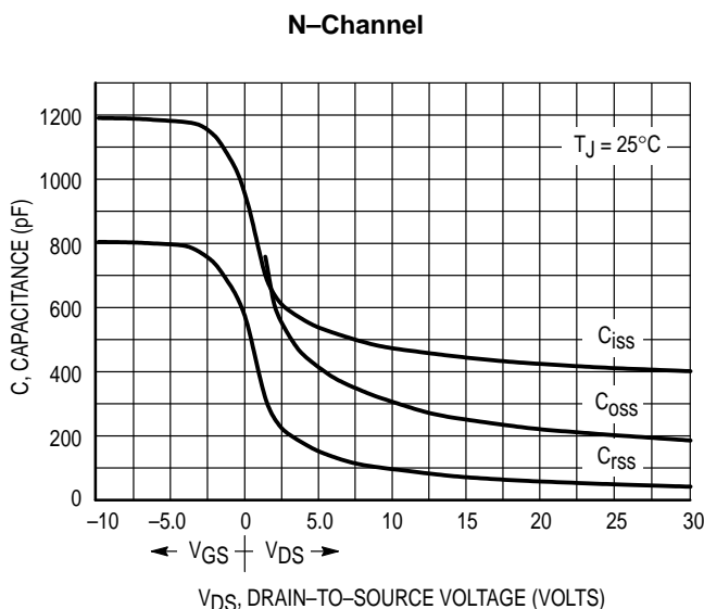
Figure 7. Capacitance Variation
