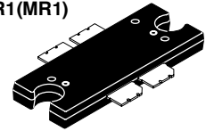
CASE 1484-02, STYLE 1 TO-272 WB-4 PLASTIC MRF6S9125NBR1(MBR1)
