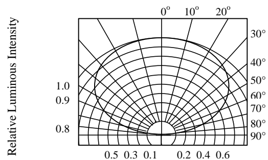
FIG.6 RADIATION DIAGRAM
