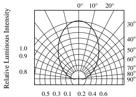
FIG.5 RADIATION DIAGRAM
