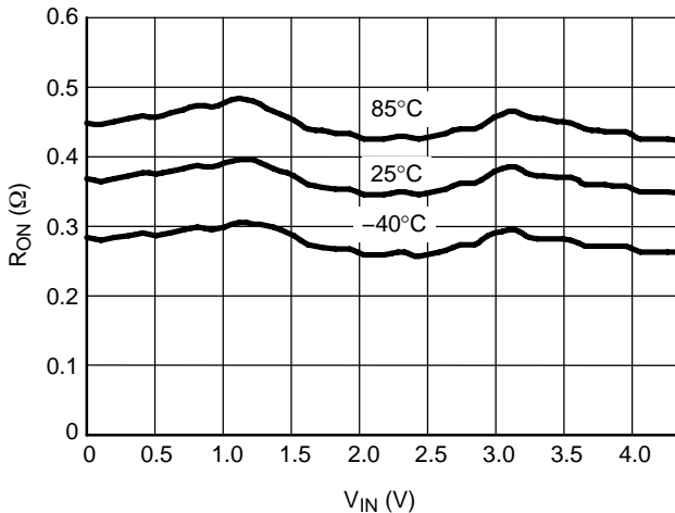
Figure 12. R_{ON} vs. V_{IN} vs. Temperature @ V_{CC} = 4.3\text{ V}
