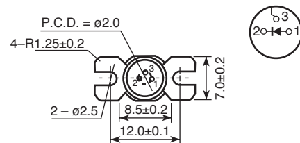
PIN CONNECTIONS
