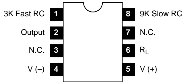
Pin Connection Diagram
