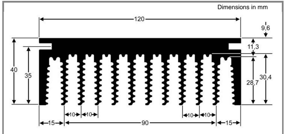
P 23 general profile dimensions (w = 0,75 kg)
