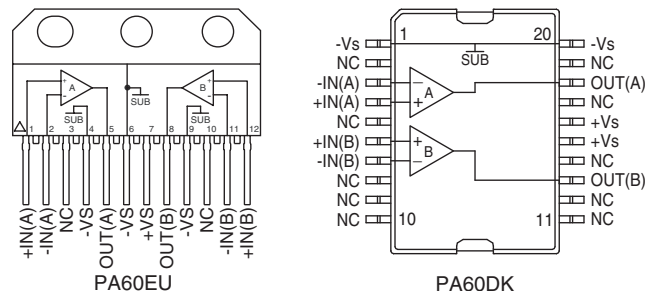
FIGURE 3. External connections
