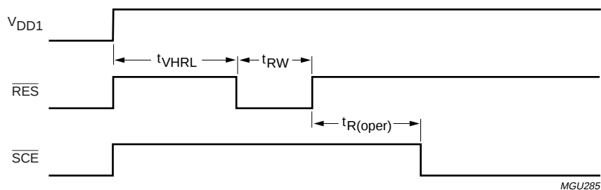
Fig.37 Reset timing.
