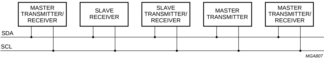
Fig.25 System configuration.
