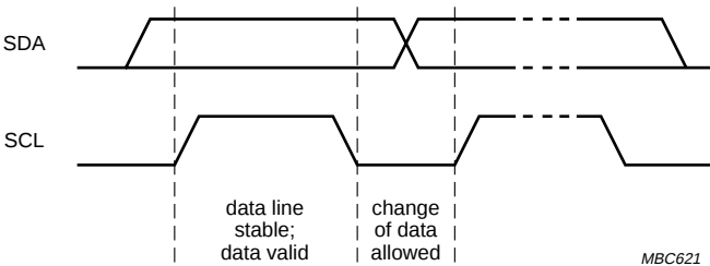
Fig.26 Bit transfer.
