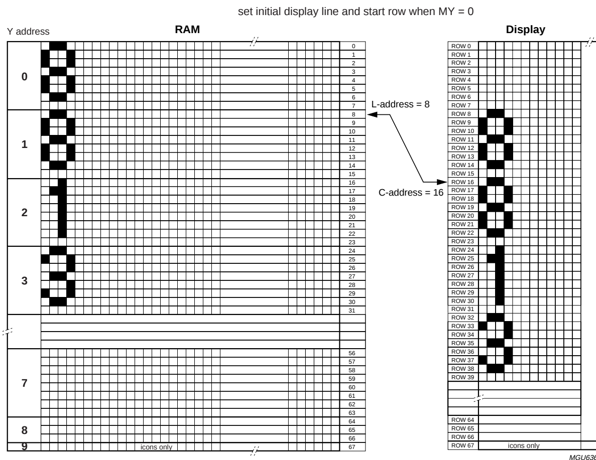
Fig.33 Effect of L address when MY = 0.
