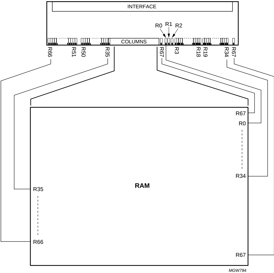
Fig.14 Row order and interconnection with BRS = 1, MY = 0 and N/\overline{P} = 1 .
