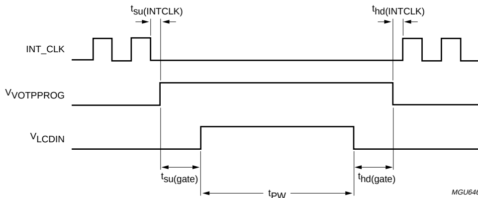
Fig.50 Programming waveforms.
