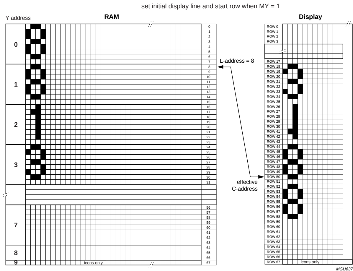
Fig.34 Effect of L address when MY = 1.
