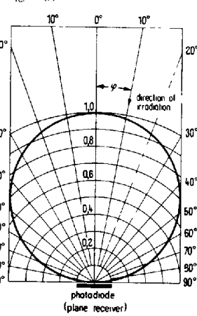
Directional characteristic
