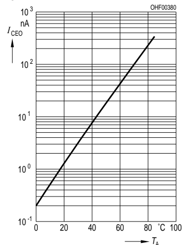
Dark Current I_{CEO} = f(T_A) V_{CE} = 20 V, E = 0
