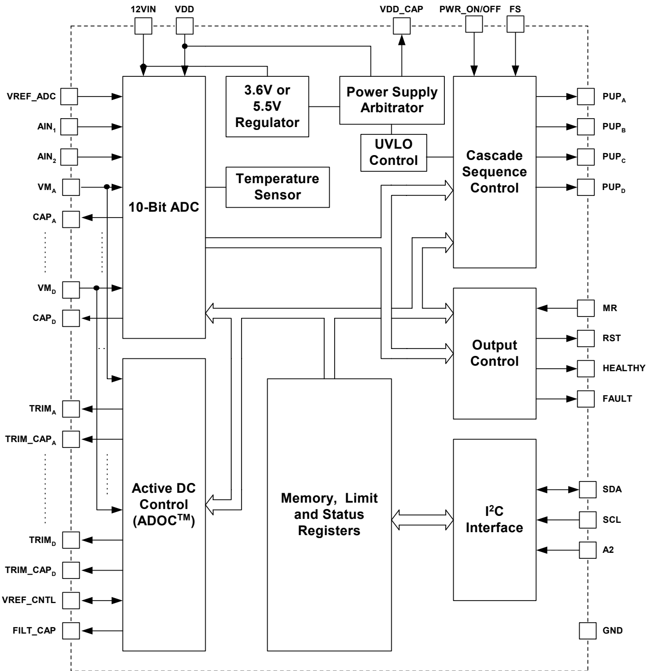
Figure 3 – SMM465 Internal Functional Block Diagram.
