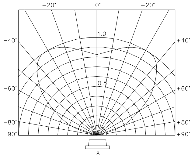
Radiation Diagram
