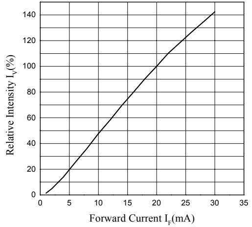
Relative Intensity I_v (%) vs Forward Current
