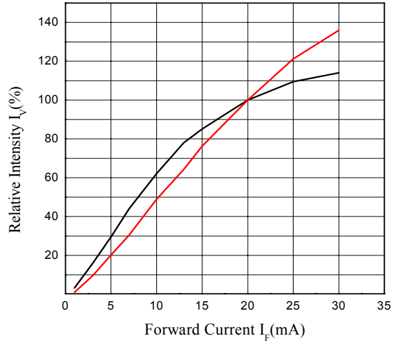
Relative Intensity I_v (%) vs Forward Current I_F (mA)
