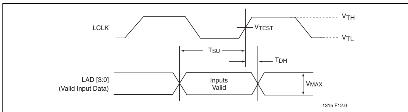
FIGURE 11: Input Timing Parameters (LPC Mode)
