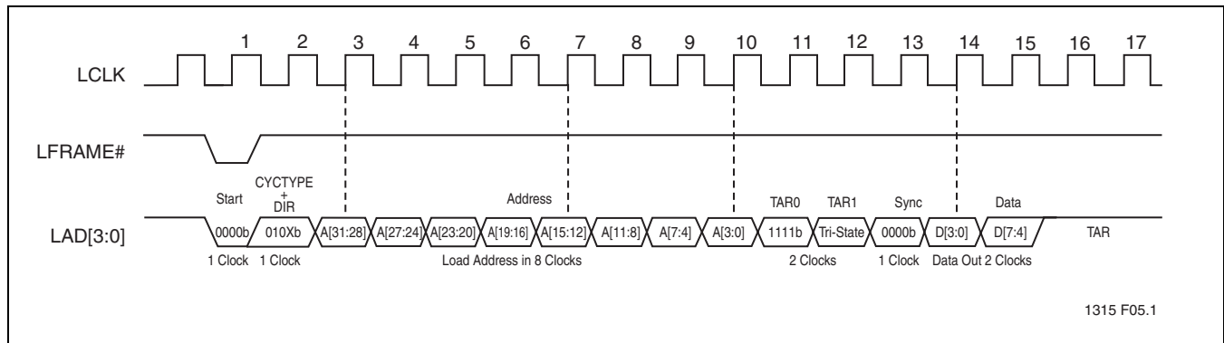
FIGURE 4: LPC MEMORY READ CYCLE WAVEFORM
