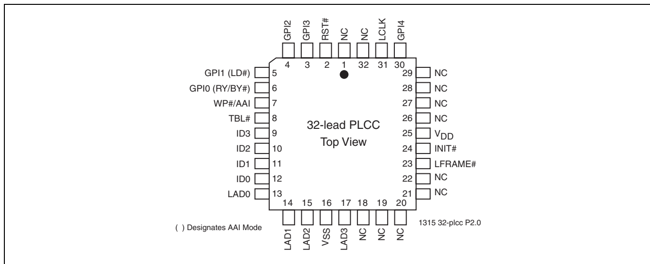
FIGURE 3: Pin Assignments for 32-lead PLCC
