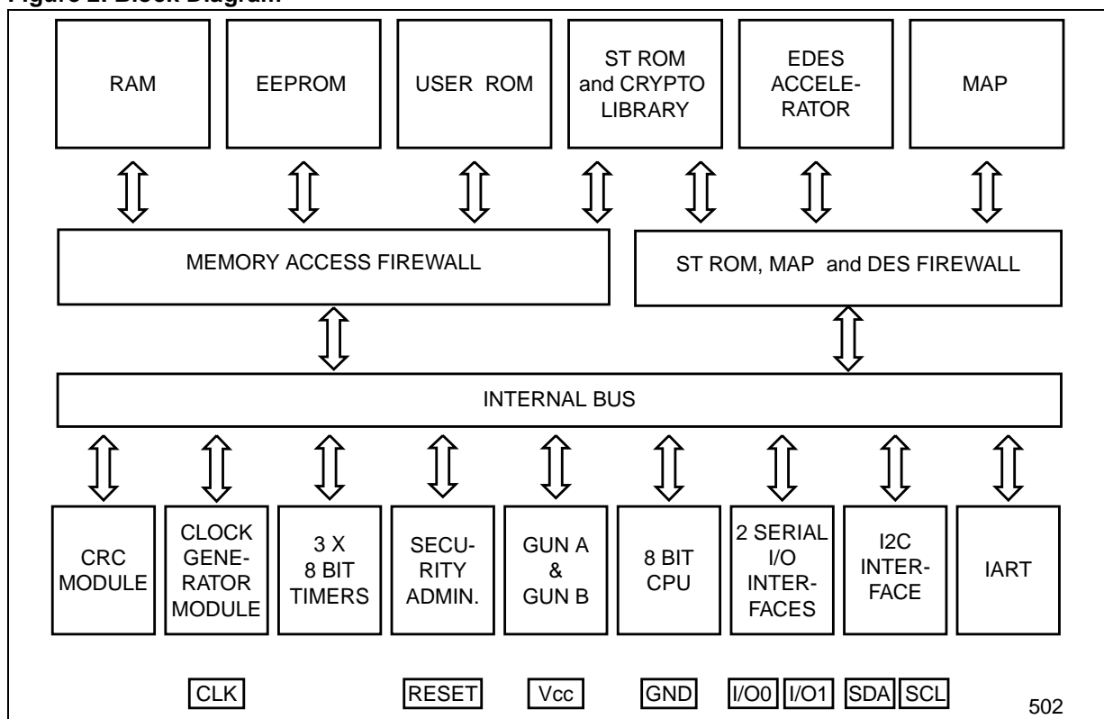
Figure 2. Block Diagram
