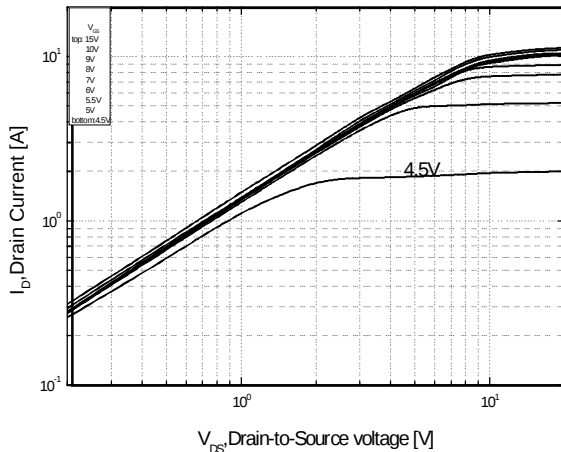
Fig 1. On-State Characteristics
