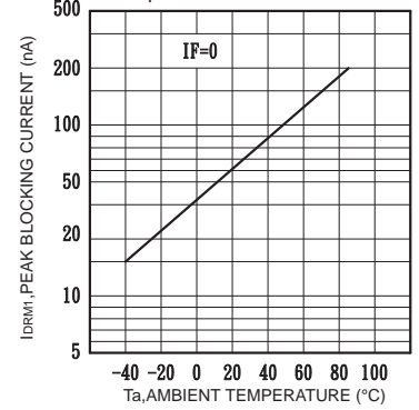
Fig.3 Leakage with LED Off versus Temperature
