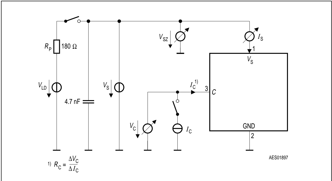
Figure 3 Test Circuit 1
