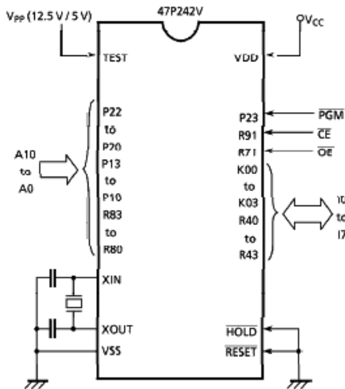
Figure 1-3. Setting for PROM mode
