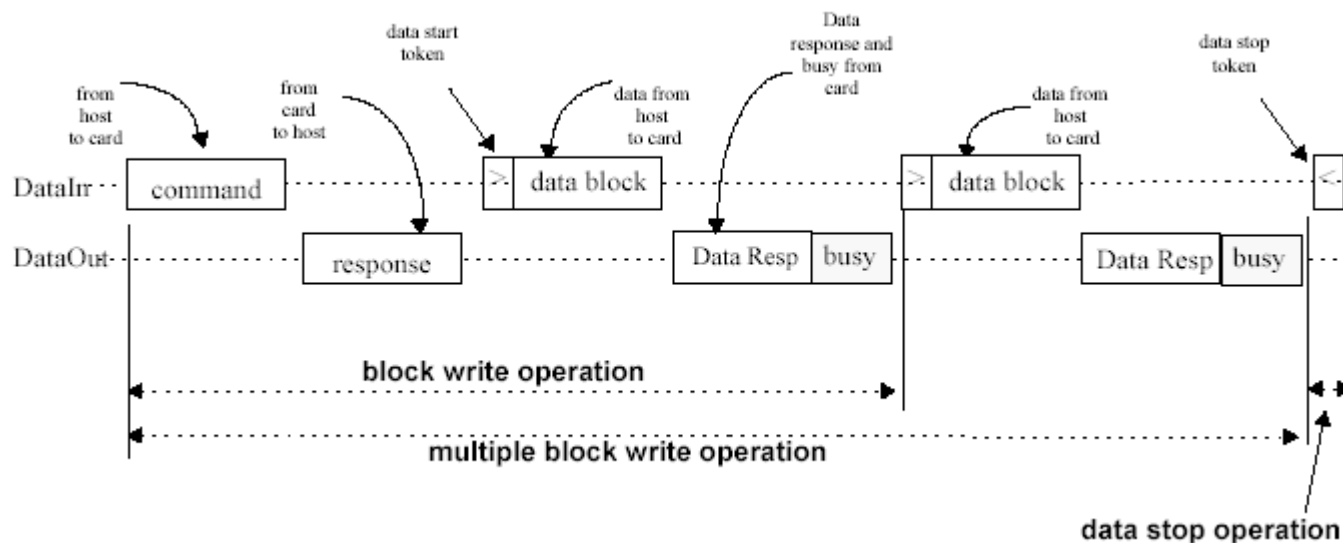
Figure 13: Write operation
