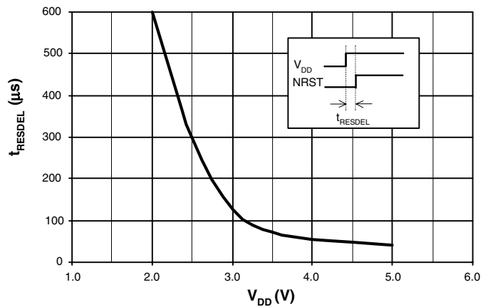
Figure 9. Typical Reset Delay After Switching V_{DD} On
