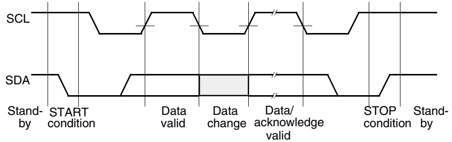
Figure 6. Serial Protocol
