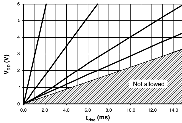
Figure 10. V_{DD} Rise Time to Ensure Power-on Reset
