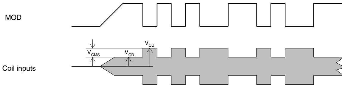
Figure 3. Modulation
