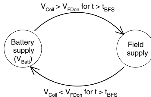
Figure 5. Switch Conditions for Power Management
