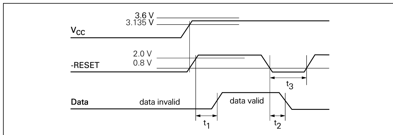
Figure 7 Timing Diagram
