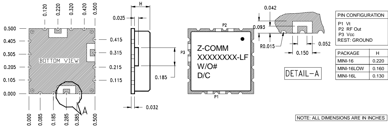
PHYSICAL DIMENSIONS
