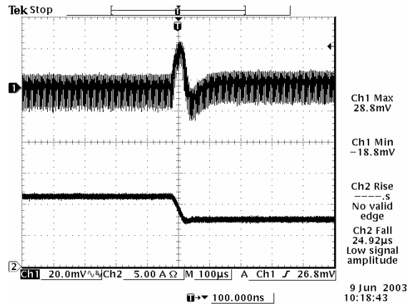
Transients 75% to 50% load, 1.25 Vdc Output
