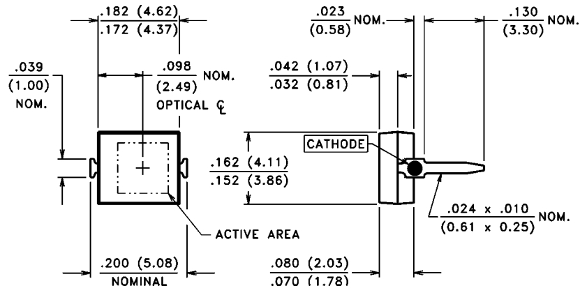
CASE 22 MINI-DIP CHIP ACTIVE AREA: .012 in 2 (7.45 mm 2 )
