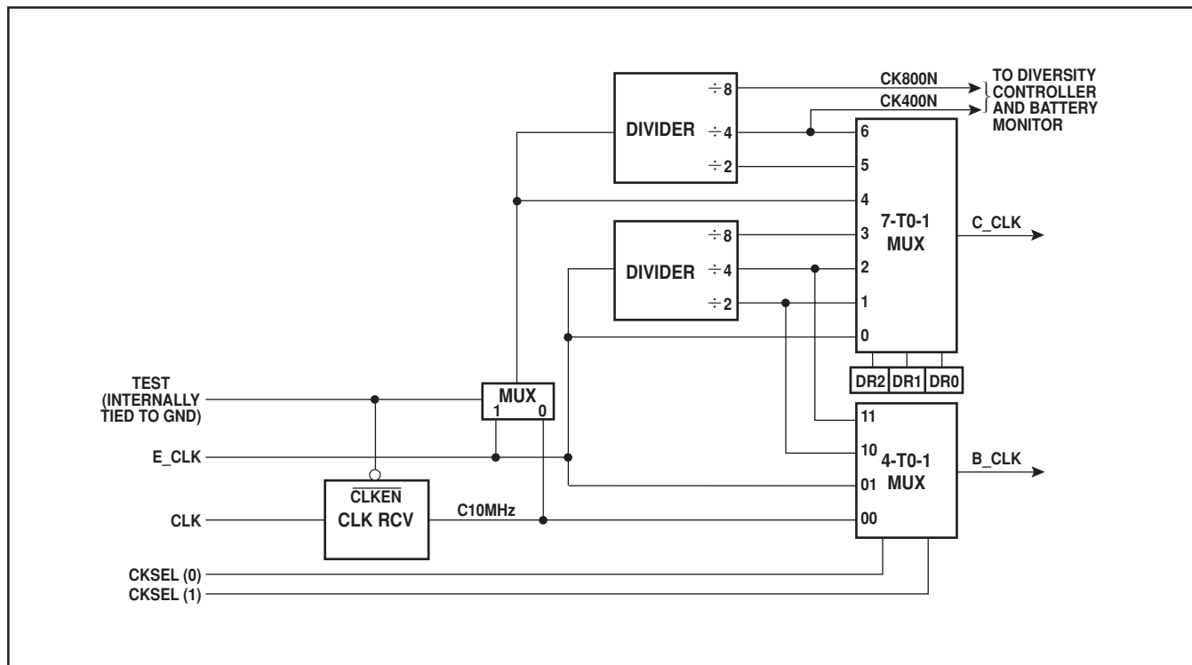
Fig. 14 Clock selector/generator
