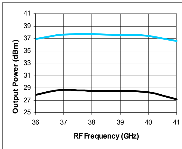
Two tone test with 18 dBm / tone — IP3 — P1 dB
