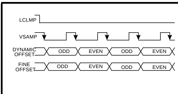
Figure 14. APOAM SYNCHRONIZATION AND REGISTER ALTERNATION
