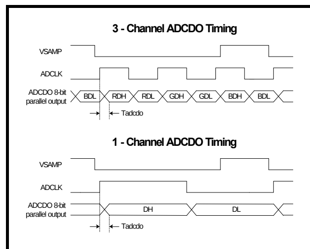
FIGURE 5. ADCDO TIMING (ADCLK POL =0, VSAMP POL =0)
