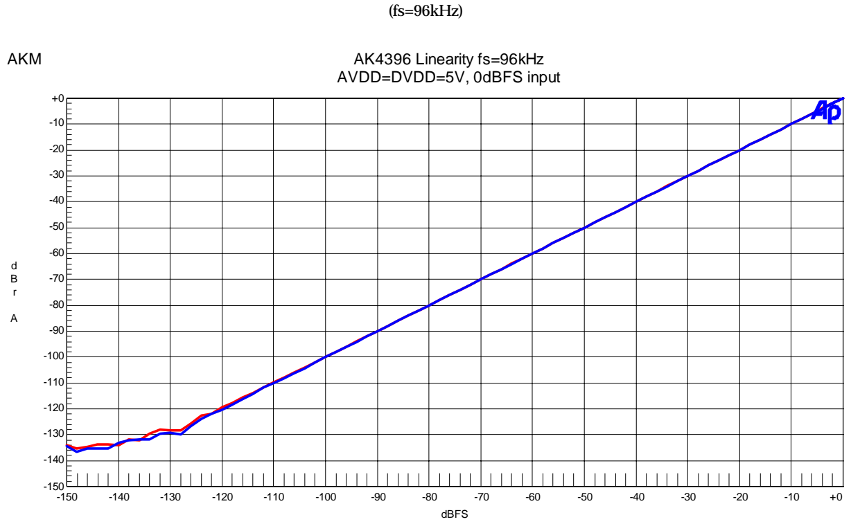
Figure 24 Linearity (fin=1kHz)
