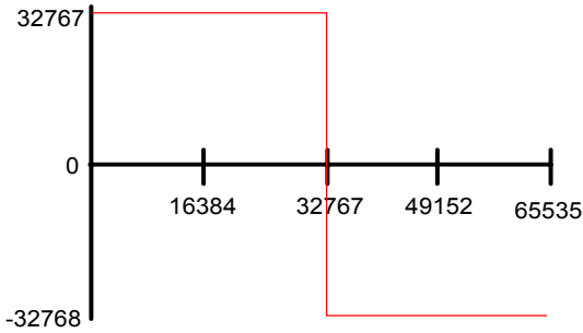
Figure 2. One period of a calculated square wave
