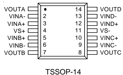
TSSOP-14
