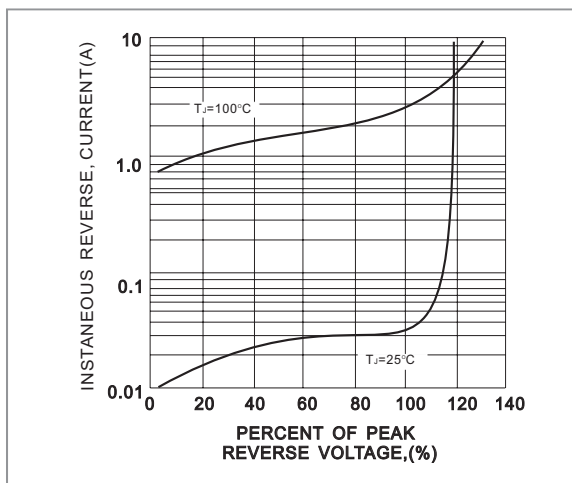
FIG. 3-TYPICAL REVERSE CHARACTERISTICS
