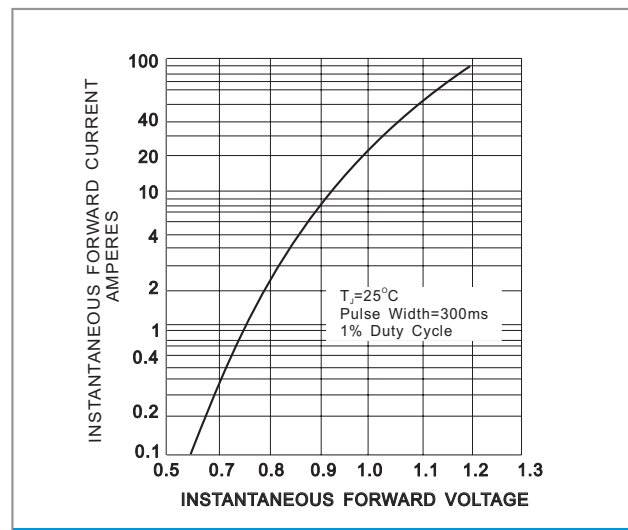
FIG. 2-TYPICAL INSTANTANEOUS FORWARD CHARACTERISTICS PER ELEMENT
