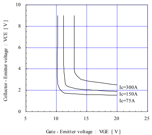
Collector-Emitter voltage vs. Gate-Emmitter voltage (typ.) Tj=25°C / chip
