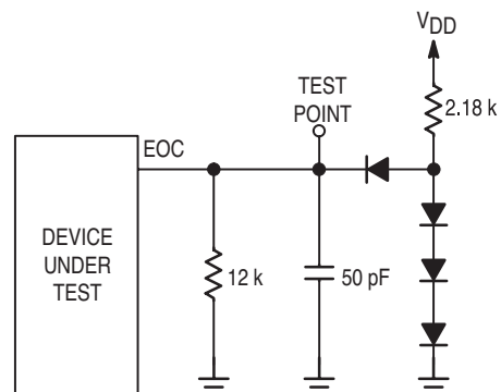
Figure 8. Test Circuit
