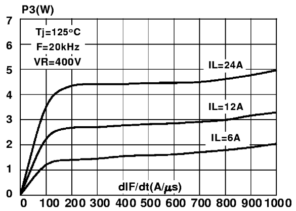
Fig 9 : Switching OFF losses versus dI/dt
