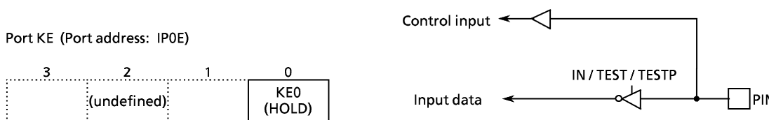
Figure 3-6. Port KE
