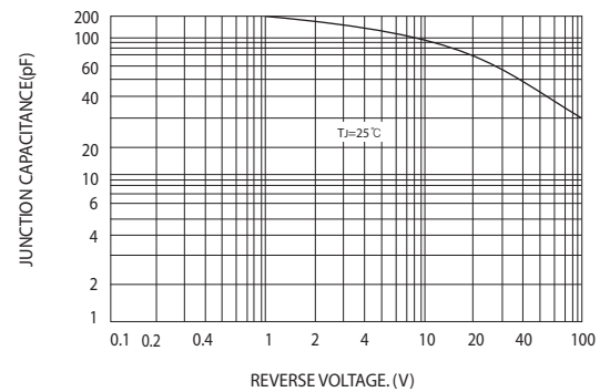
FIG.4-TYPICAL JUNCTION CAPACITANCE
