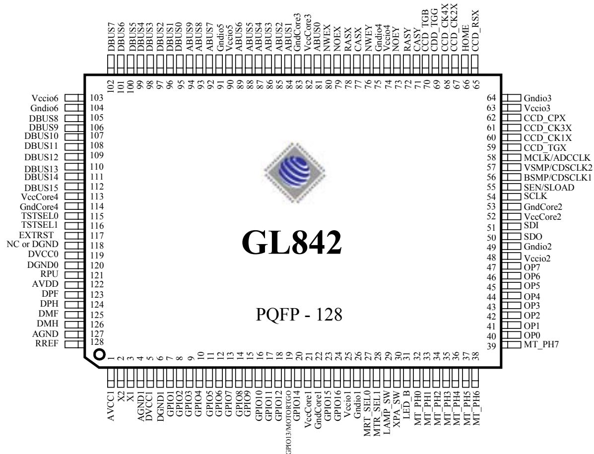
Figure 3.1 - Pinout Diagram
