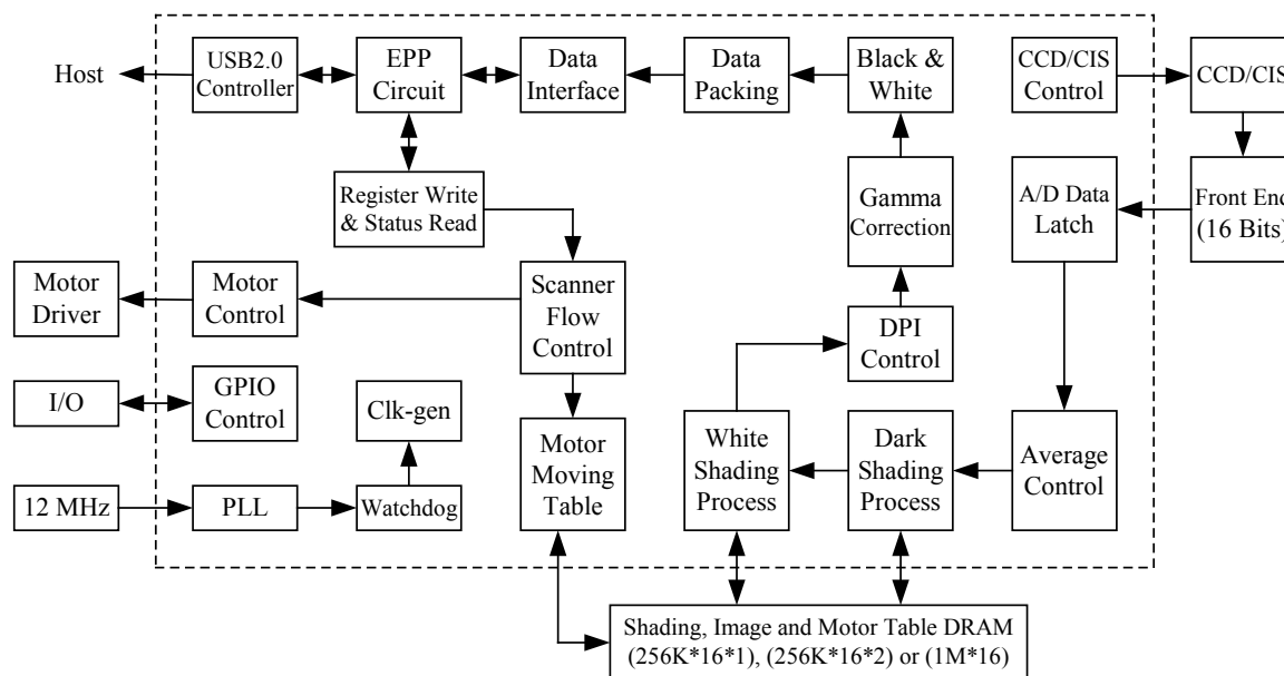
Figure 5.2 - Function Block Diagram
