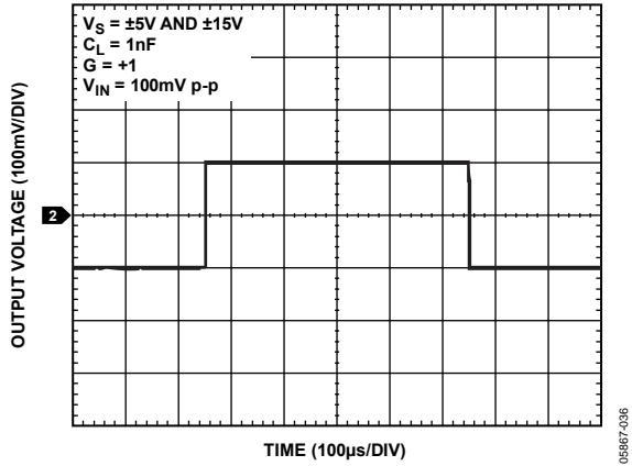
Figure 33. Small-Signal Transient
