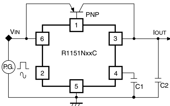
Fig.3 Ripple Rejection, Line Transient Response Test Circuit C1=220pF , C2=10\mu F
