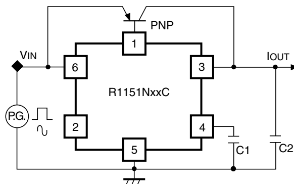
Fig.4 Load Transient Response Test Circuit C1=220pF , C2=10\mu F
