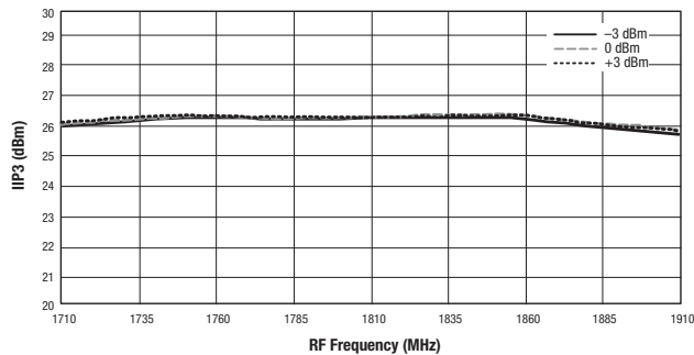
Figure 20. Mixer B IIP3 vs Frequency and LO Power
