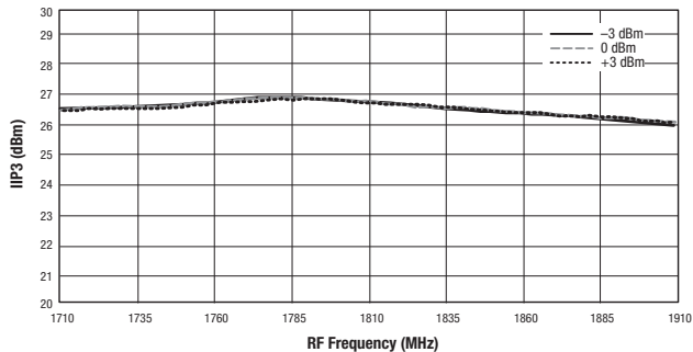
Figure 17. Mixer A IIP3 vs Frequency and LO Power
