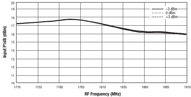
Figure 23. Mixer A Input P1dB vs Frequency and LO Power
