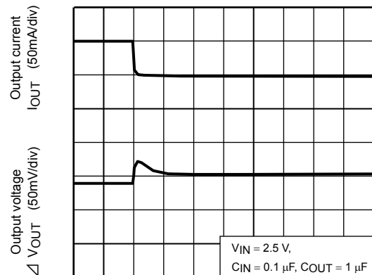
TCR5SB15 ( I_{OUT} = 100\text{m to }50\text{mA} )
