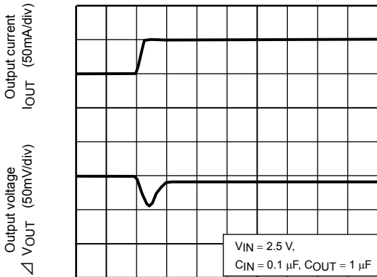
TCR5SB15 ( I_{OUT} = 50\text{m to }100\text{mA} )
