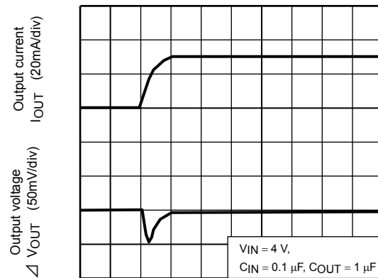
TCR5SB30 ( I_{OUT} = 1\text{m to }30\text{mA} )
