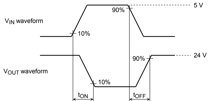
Measured Waveforms
