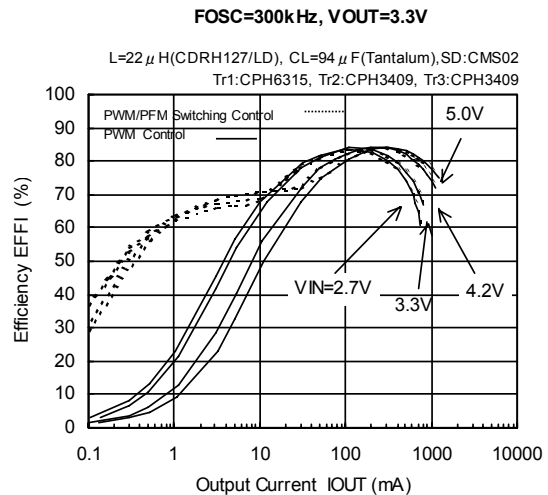
(2) Efficiency vs. Output Current
