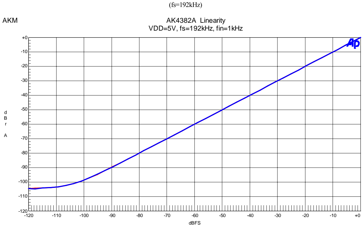
Figure 33. Linearity (fin=1kHz)
