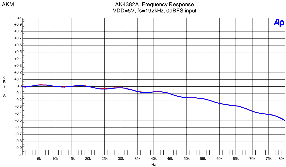
Figure 34. Frequency Response (0dBFS input)
