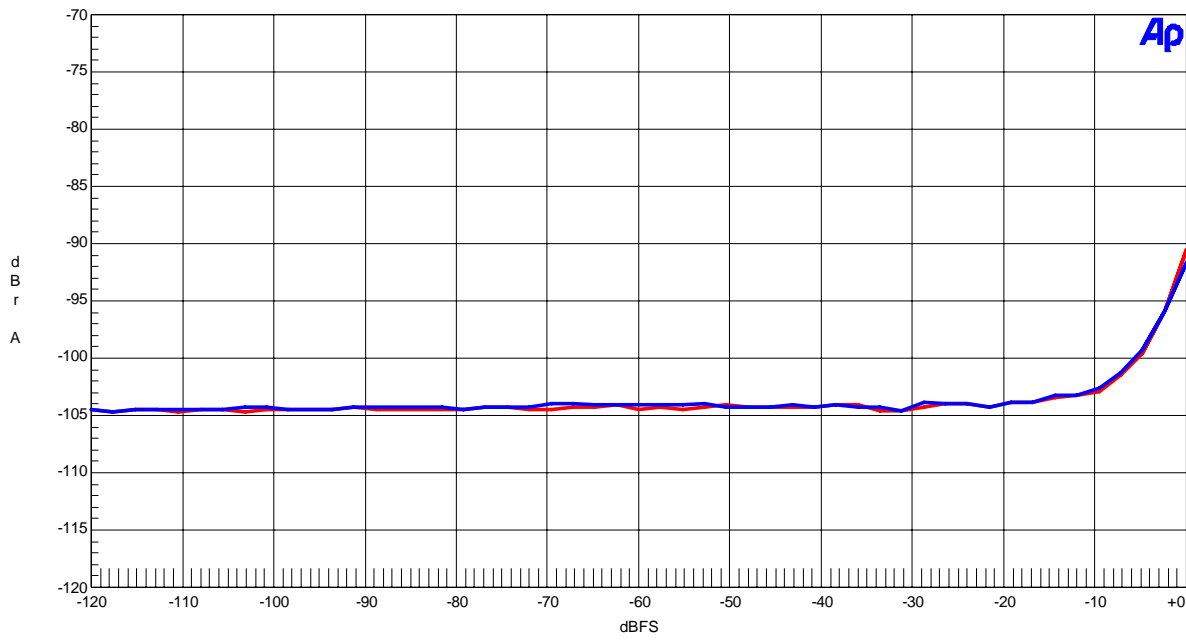
Figure 31. THD+N vs. Input level (fin=1kHz)
